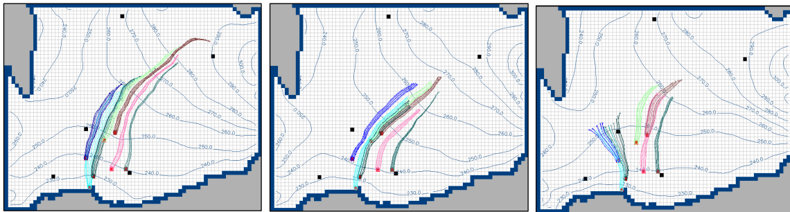
Fig. 5 Extended protection zones obtained with new K heterogeneous distributions and t = 3500 days, showing the uncertainty related to the distribution of K and the influence of this parameter in pathlines and travel times of pollutant particles
