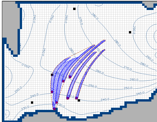
Fig. 4 Pathlines for t = 3500 days (extended protection zones)
